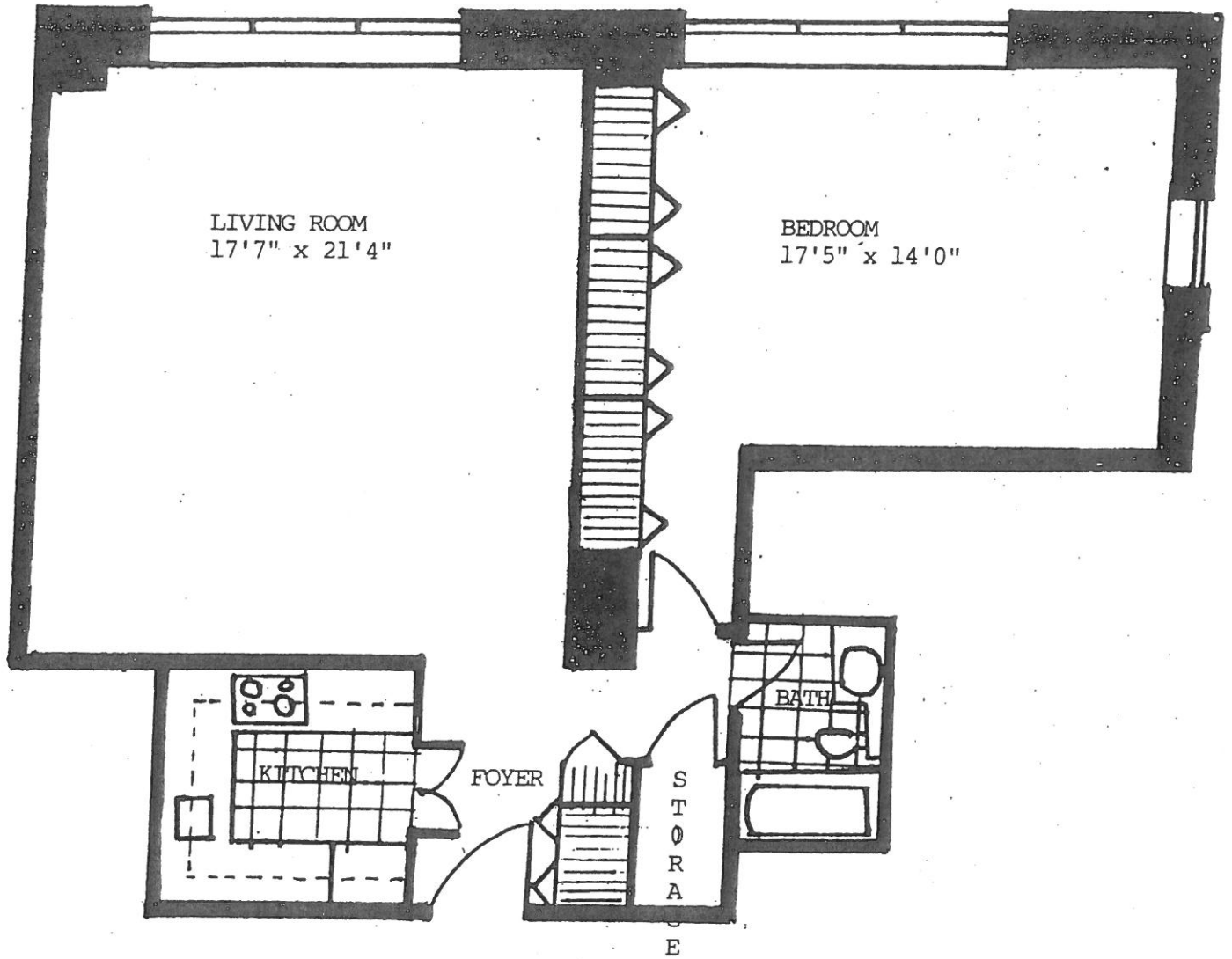
TYPICAL ONE BEDROOM FLOOR PLAN '08 - EAST SIDE
