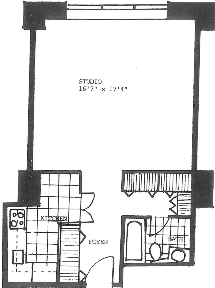
TYPICAL STUDIO FLOOR PLAN '04 - EAST SIDE
